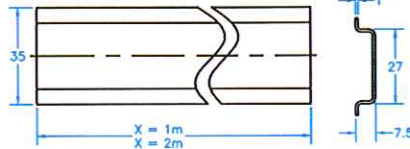
Unperforated Dimensions
